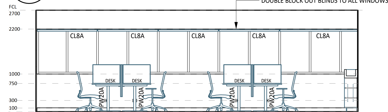
9 ELEVATION DETAIL
