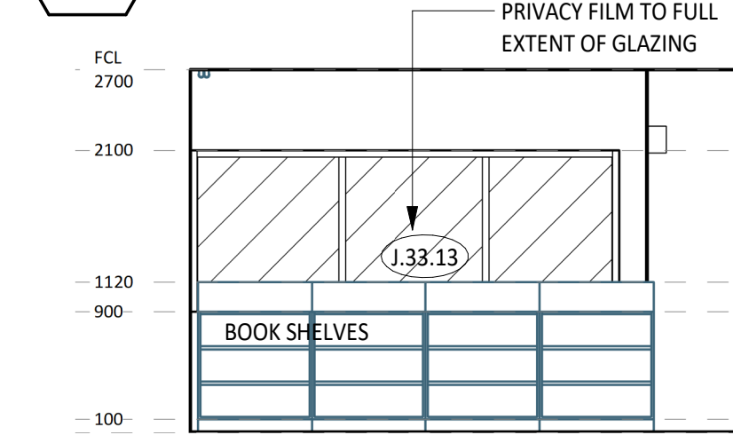
2 ELEVATION DETAIL
