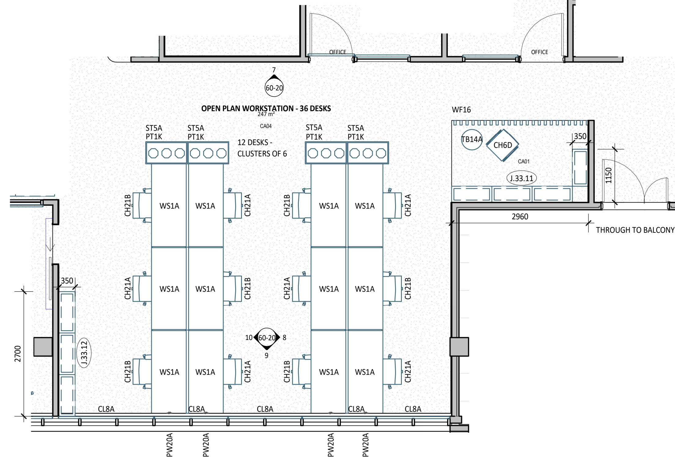
6 PLAN DETAIL
