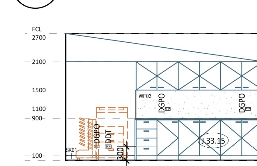
3 ELEVATION - SHARED PRINT
