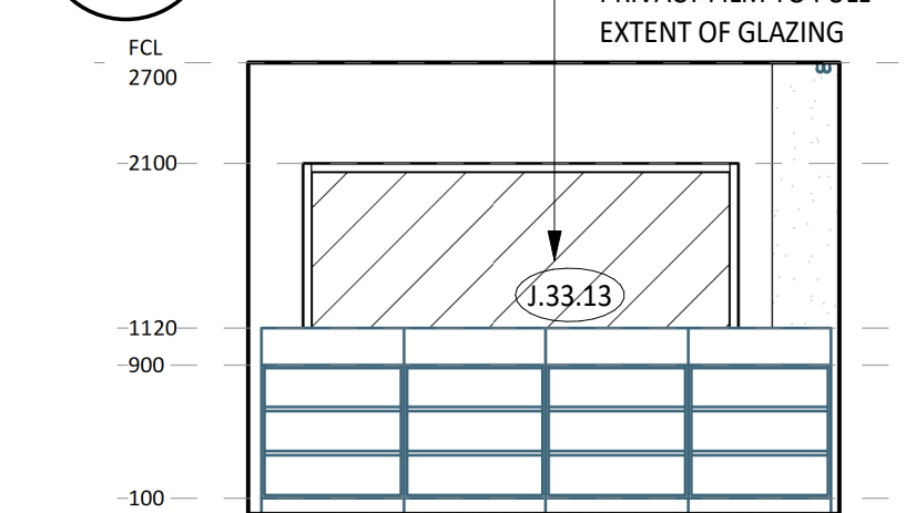
4 ELEVATION DETAIL
